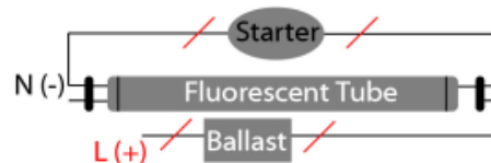
Magnetic Ballast
