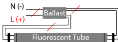
Electronic Ballast
